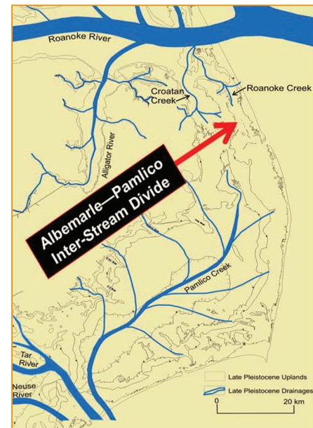
• FIGURE 11: THIS MAP SHOWS THE MAJOR INTER-STREAM DIVIDE ABOUT 9,000 YEARS AGO, WHEN SEA LEVEL WAS SUBSTANTIALLY LOWER. PAMLICO CREEK, CROATAN CREEK, AND ROANOKE RIVER WERE PRE-CUSERS OF PAMLICO SOUND, CROATAN SOUND, AND ALBEMARLE SOUND RESPECTIVELY. FOR REFERENCE ONLY, THE FIGURE INCLUDES THE OUTER BANKS, WHICH DID NOT THEN EXIST.
