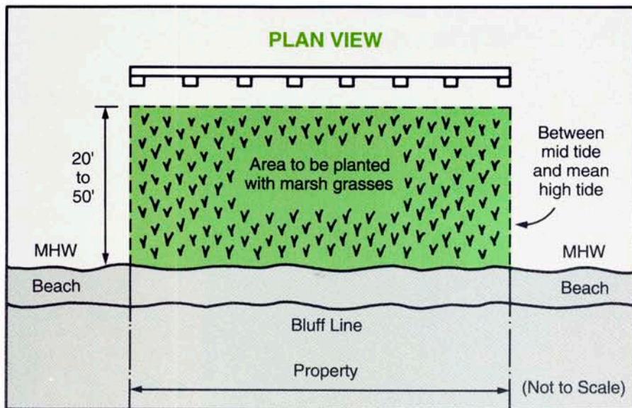
Figure 10. Layout of breakwater and planted marsh grasses.
