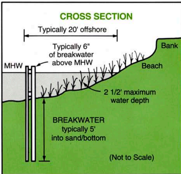
Figure 9. Breakwater cross section.
